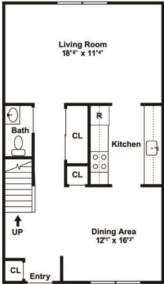
LOWER LEVEL
